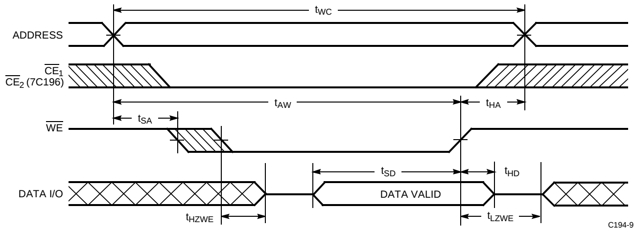
Write Cycle No. 3 ( \overline{WE} Controlled, \overline{OE} LOW) [15, 16]
