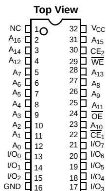
Figure 3. 32-pin SOIC pinout [1]
