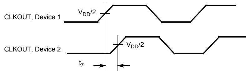
Figure 9. Device-Device Skew
