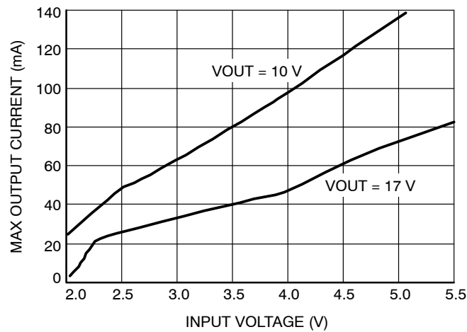
Figure 22. Maximum Output Current vs. Input Voltage
