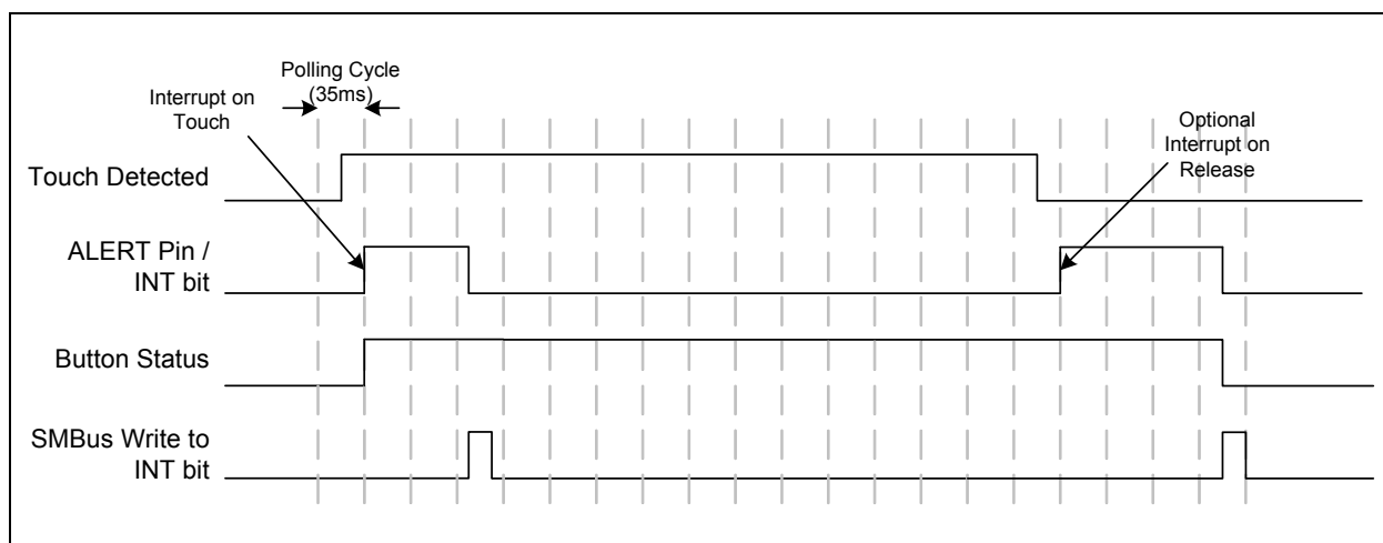
Figure 5.3 Button Interrupt Behavior - No Repeat Rate Enabled
