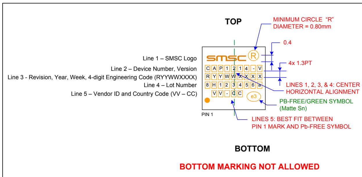
Figure 7.7 Package Markings
