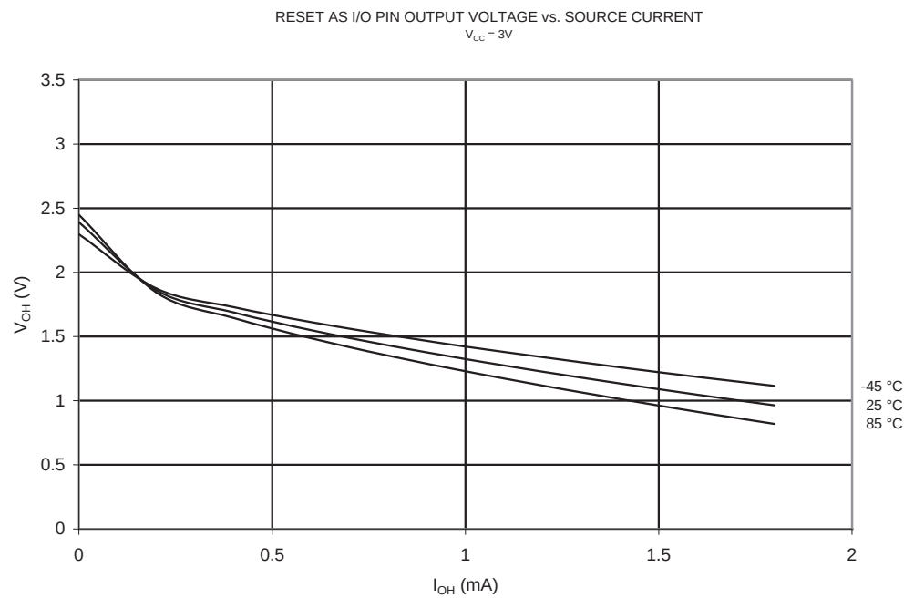
Figure 20-25. Reset Pin Output Voltage vs. Source Current ( V_{CC} = 3V )
