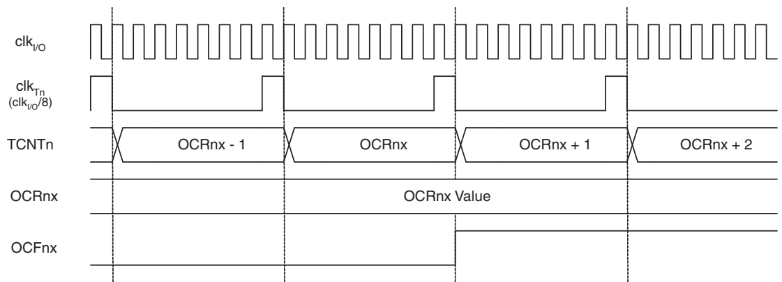
Figure 11-9. Timer/Counter Timing Diagram, Setting of OCF0x, with Prescaler ( f_{\text{clk\_I/O}}/8 )
