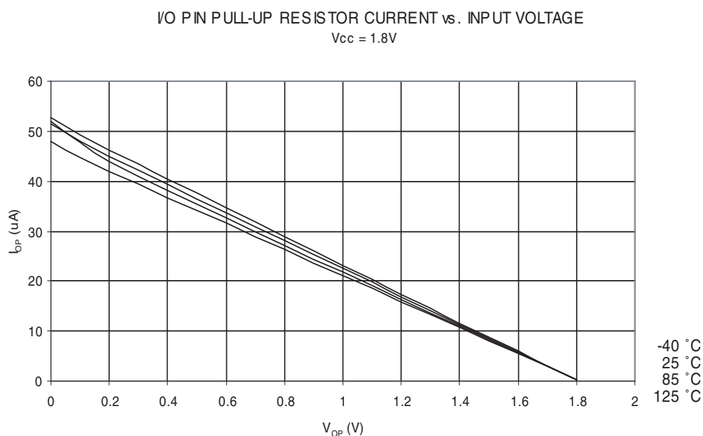
Figure 23-13. I/O Pin Pull-Up Resistor Current vs. Input Voltage ( V_{CC} = 1.8V )
