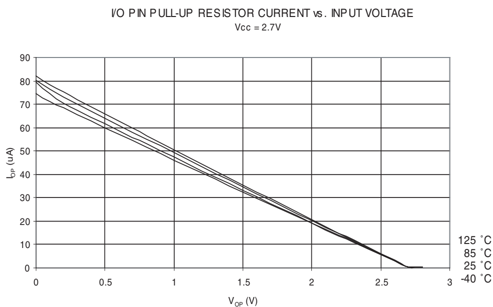
Figure 23-14. I/O Pin Pull-Up Resistor Current vs. Input Voltage ( V_{CC} = 2.7V )
