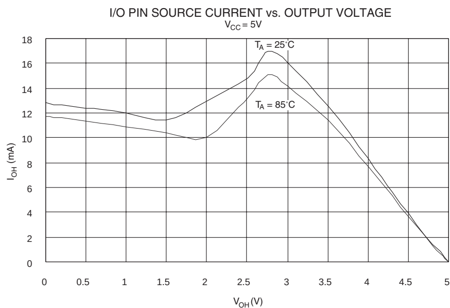
Figure 51. I/O Pin Source Current vs. Output Voltage
