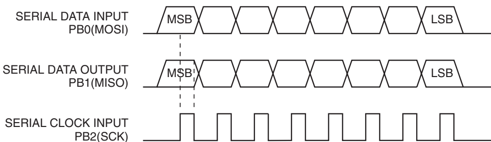
Figure 30. Low-voltage Serial Programming Waveforms
