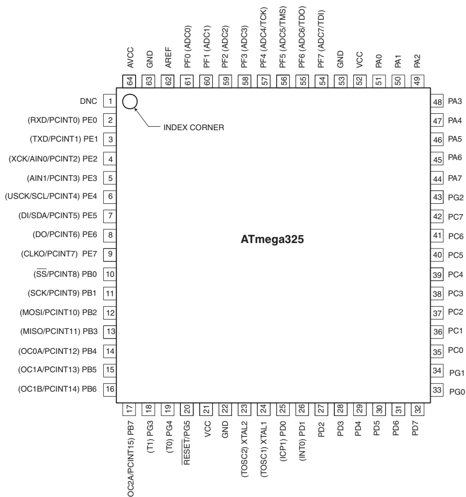
Figure 1-2. Pinout ATmega325P
