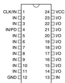
Figure 1-4. DIP/SOIC
