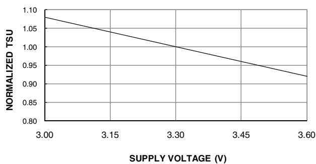
NORMALIZED T_{SU} VS. V_{CC}
