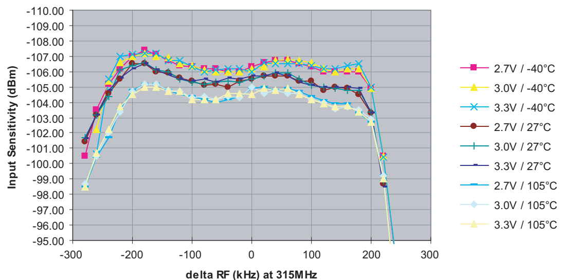
Figure 2-5. Measured Sensitivity (315MHz, FSK, 9.6Kbits/s, \pm 38 kHz, Manchester) Versus Frequency Offset Input Sensitivity (dBm) at BER < 1e-3, ATA5746C, FSK, 9.6Kbits/s (Manchester), BR = 2
