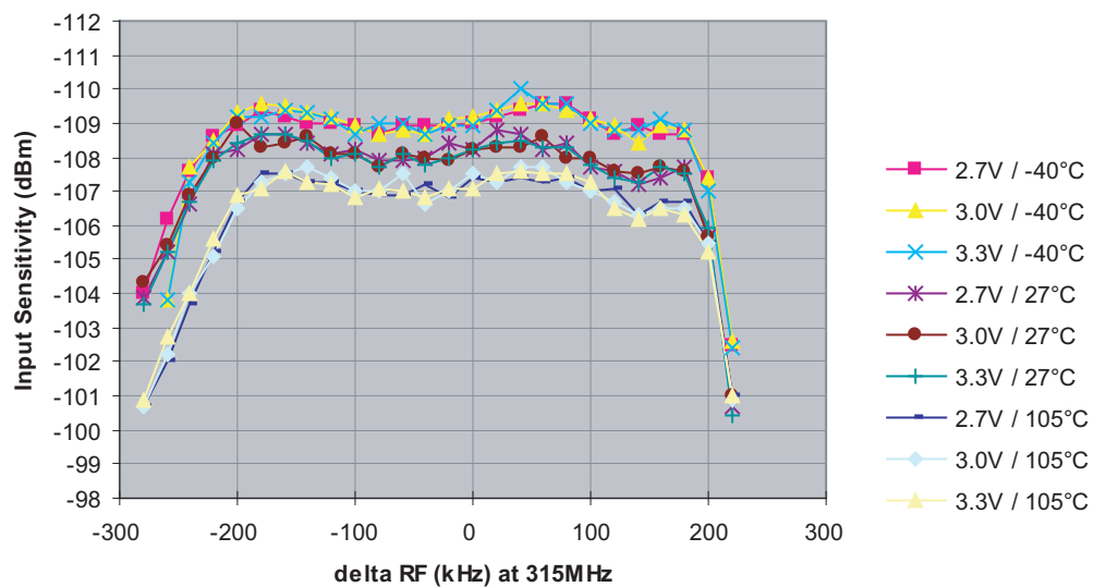
Figure 2-5. Measured Sensitivity (315MHz, FSK, 9.6Kbits/s, \pm 38 kHz, Manchester) Versus Frequency Offset Input Sensitivity (dBm) at BER < 1e-3, ATA5746C, FSK, 9.6Kbits/s (Manchester), BR = 2
