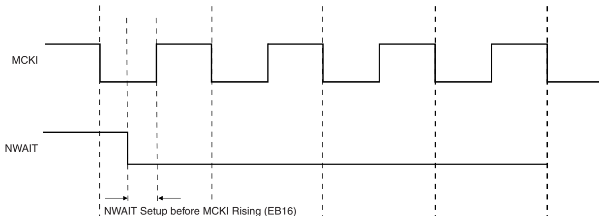
Figure 24-1. NWAIT Rising
