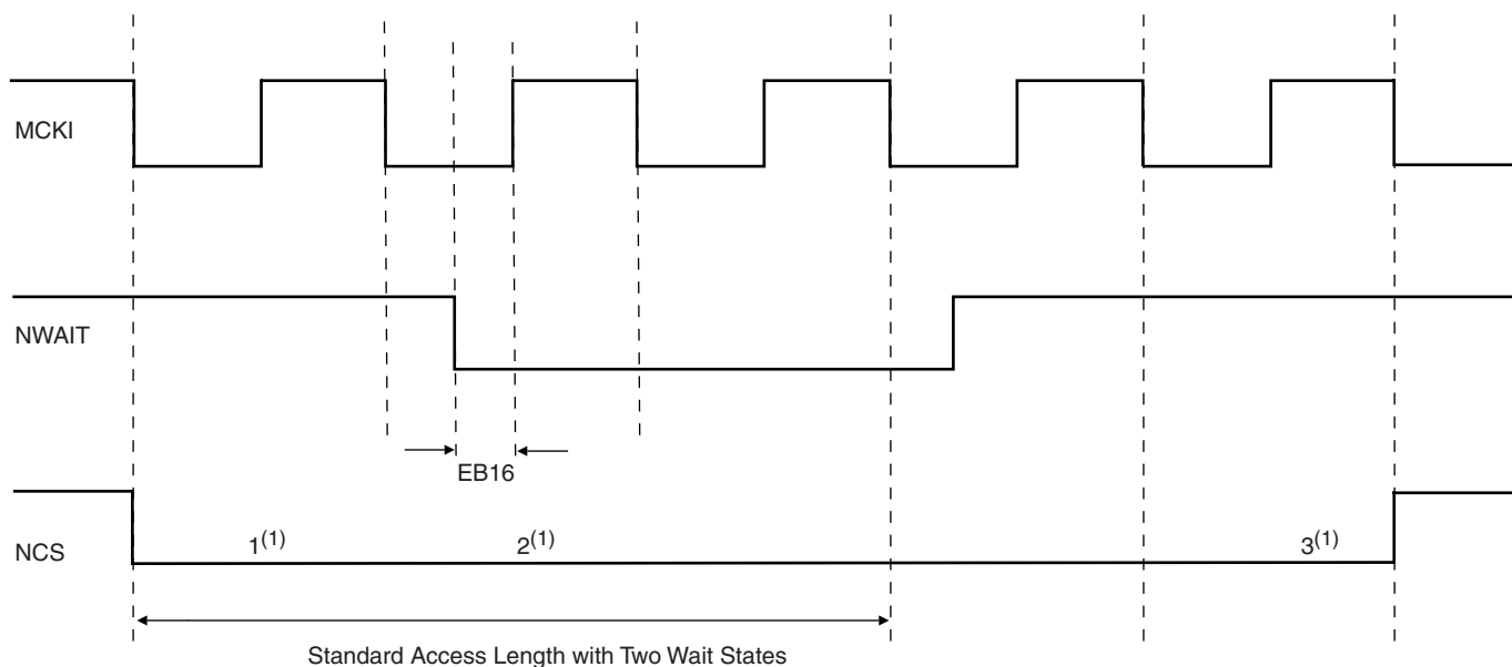
Figure 24-2. Number of Standard Wait States is Two
