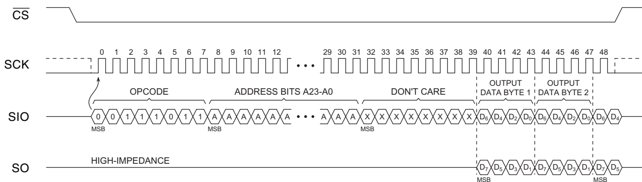
Figure 7-4. Dual-Output Read Array
