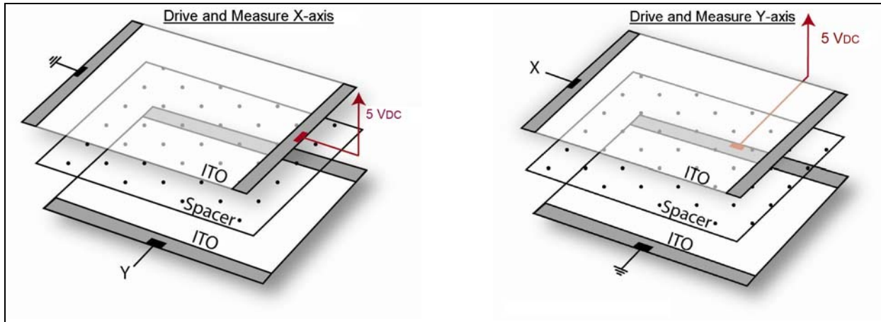
FIGURE 2-1: 4-WIRE DECODING
