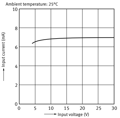
10. Input current vs. input voltage characteristics
