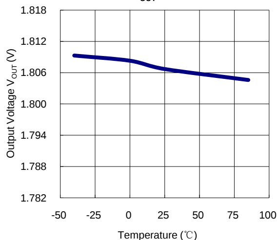
Output Voltage vs. Temperature V_{OUT}=1.8V
