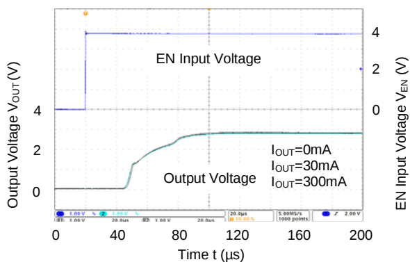
Turn On Waveforms V_{OUT}=2.8V
