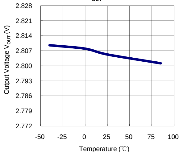
Output Voltage vs. Temperature V_{OUT}=2.8V
