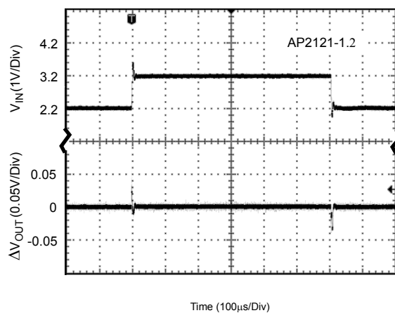
Figure 19. Line Transient (Conditions: I_{\text{OUT}} = 30\text{mA} , C_{\text{IN}} = 1\mu\text{F} , C_{\text{OUT}} = 1\mu\text{F} )
