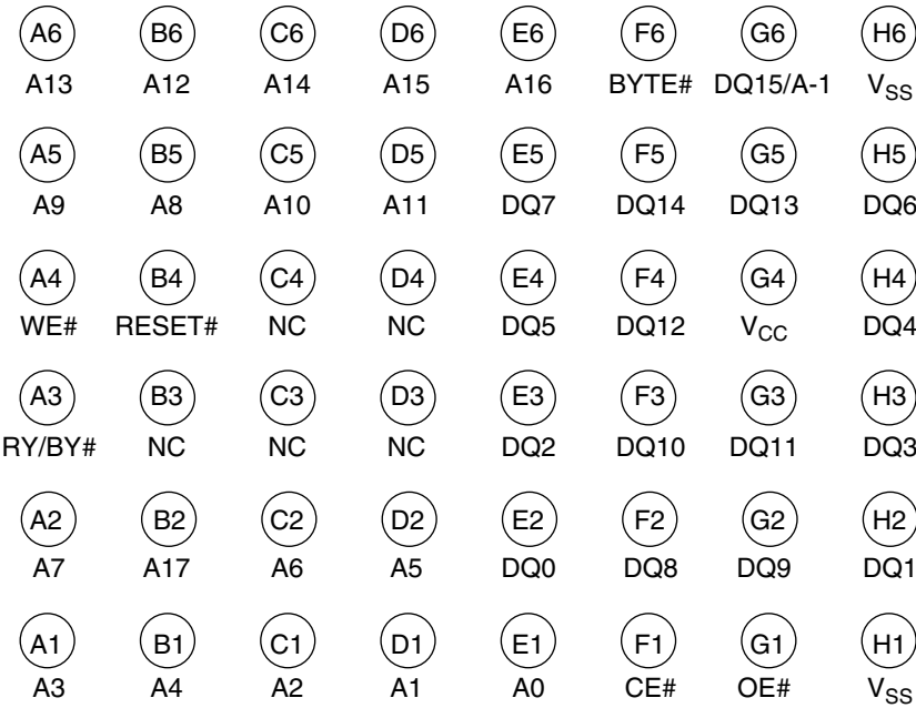
FBGA Top View, Balls Facing Down
