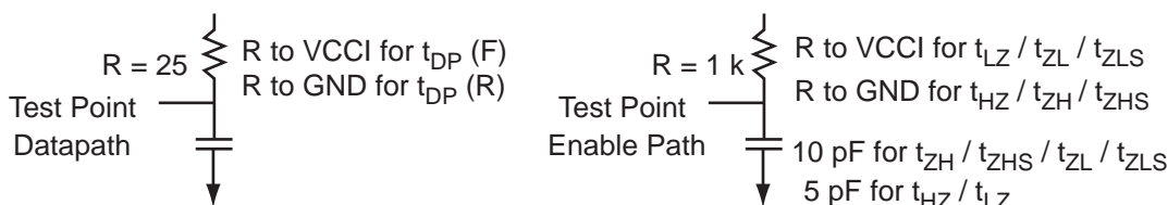
Figure 2-12 • AC Loading
