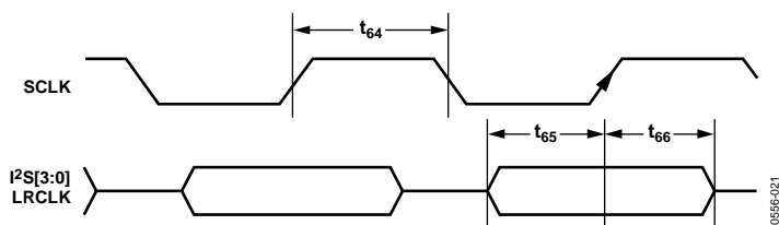
Figure 22. I²S Timing
