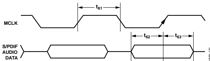
Figure 20. S/PDIF Input Timing, Data Latched on Rising Edge
