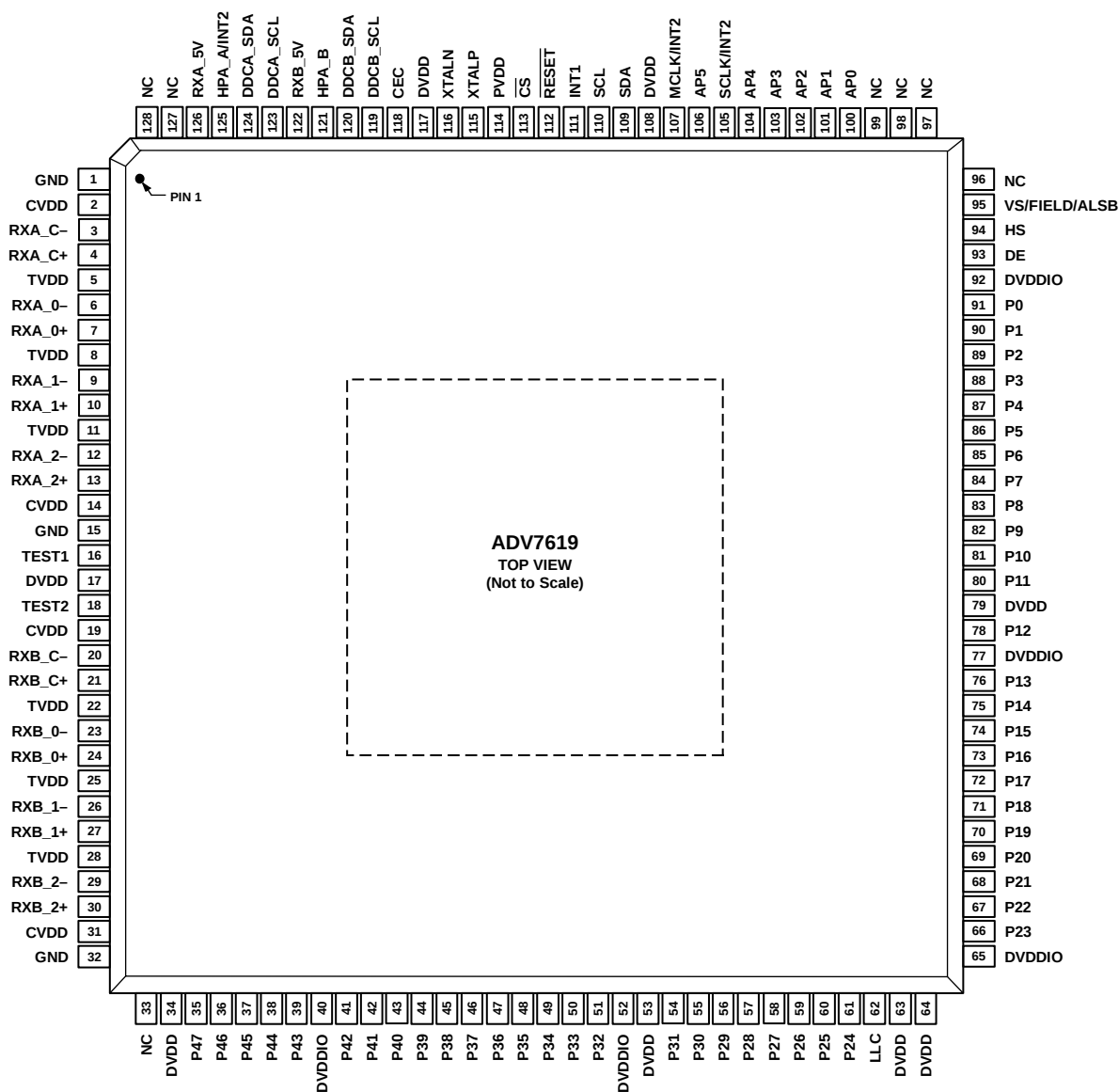
Figure 6. Pin Configuration
