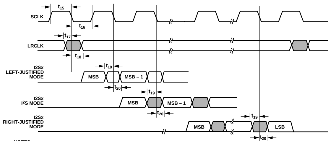
Figure 5. I²S Timing
