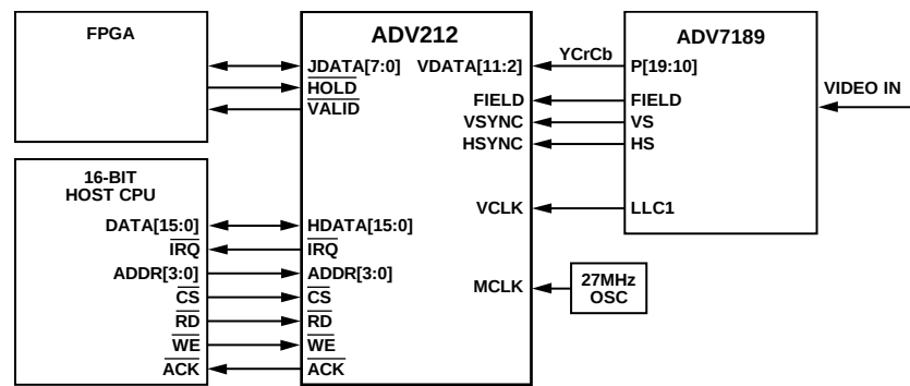
Figure 39. JDATA Application
