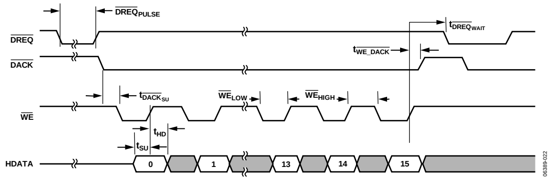
Figure 13. Burst Write Cycle for \overline{\text{DREQ}} /DMA Mode for Assigned DMA Channel (EDMOD0/EDMOD1[14:1] Not Programmed to a Value of 0000)
