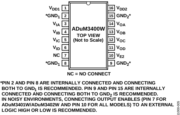
Figure 5. ADuM3400W Pin Configuration
