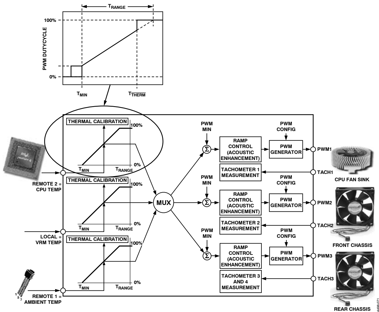
Figure 68. The T_{HYST} Value Applies to Fan On/Off Hysteresis and THERM Hysteresis
