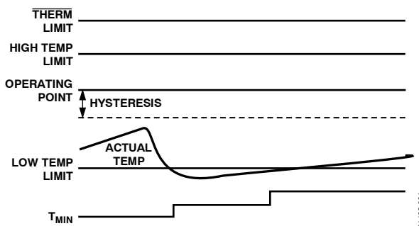
Figure 74. Increasing T_{MIN} for Quiet Operation
