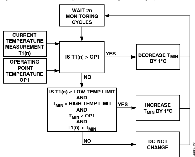
Figure 71. Long Cycle Steps
