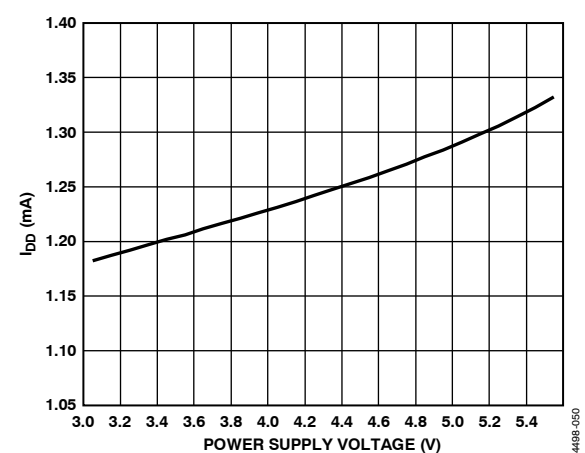
Figure 9. Normal I_{DD} vs. Power Supply
