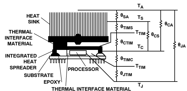
Figure 51. Thermal Model
