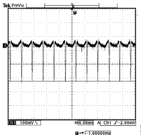
Figure 40. Fan Speed Sensing Waveform at TACHx Pin
