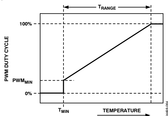
Figure 61. T_{\text{RANGE}} Parameter Affects Cooling Slope
