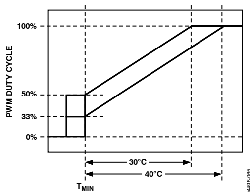
Figure 62. Adjusting \text{PWM}_{\text{MIN}} Affects T_{\text{RANGE}}
