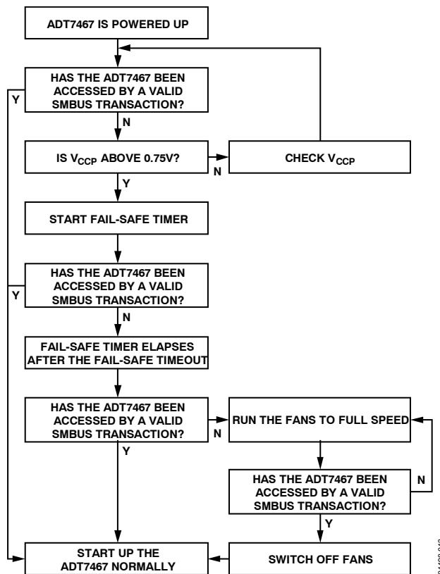
Figure 48. Power-On Flowchart
