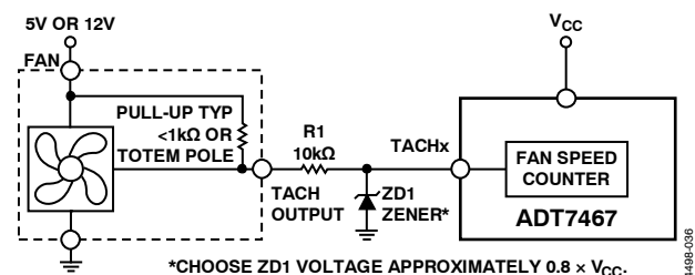
Figure 44. Fan with Strong TACH Pull-Up to >V_{CC} or Totem-Pole Output,
