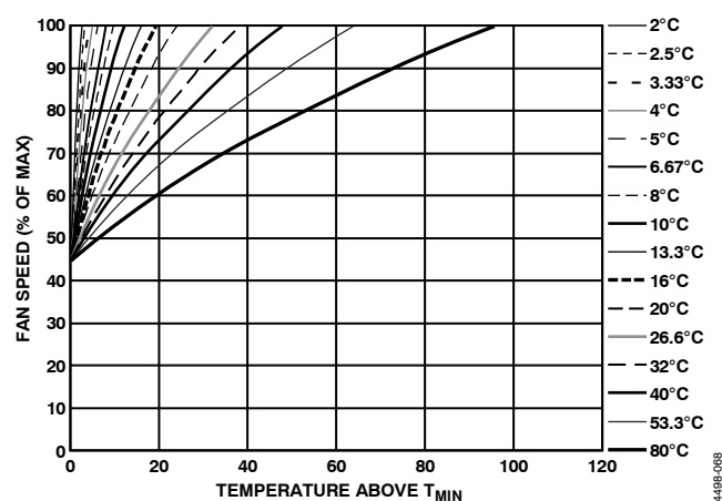
Figure 65. T_{\text{RANGE}} and Percentage of Fan Speed Slopes with \text{PWM}_{\text{MIN}} = 20\%
