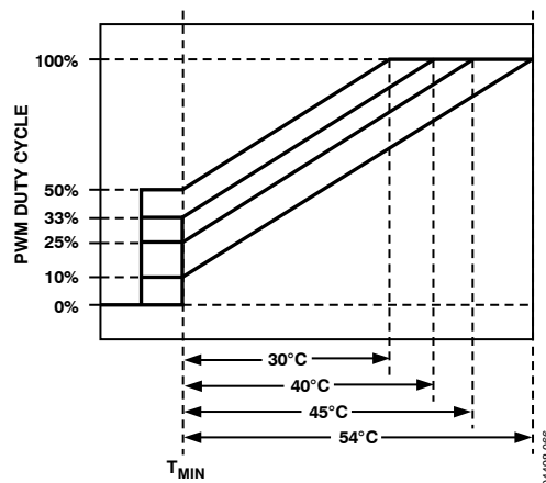
Figure 63. Increasing \text{PWM}_{\text{MIN}} Changes Effective T_{\text{RANGE}}
