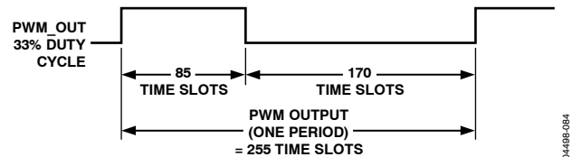
Figure 82. 33% PWM Duty Cycle, Represented in Time Slots
