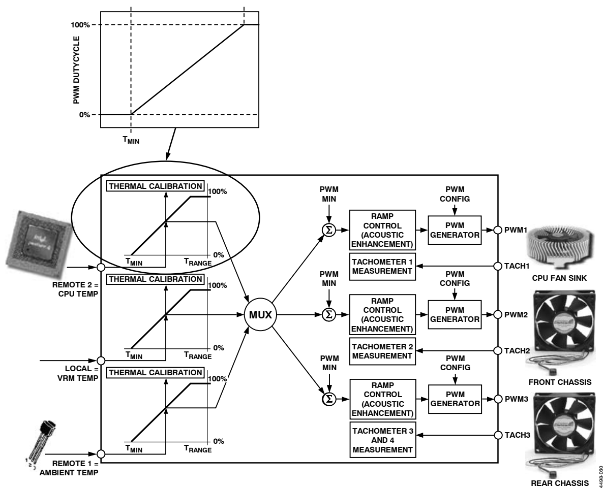
Figure 57. Understanding the T_{MIN} Parameter
