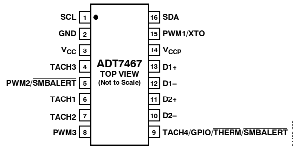
Figure 3. Pin Configuration
