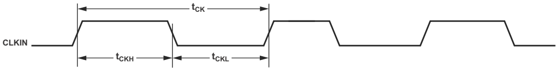
Figure 6. Clock Input
