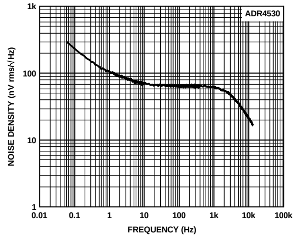
Figure 47. ADR4530 Output Noise Spectral Density
