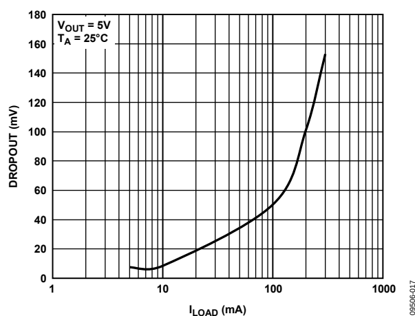
Figure 21. Dropout Voltage vs. Load Current, V_{OUT} = 5\text{ V}
