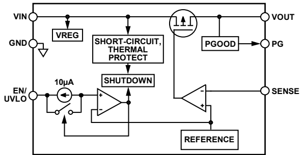
Figure 60. Fixed Output Voltage Internal Block Diagram
