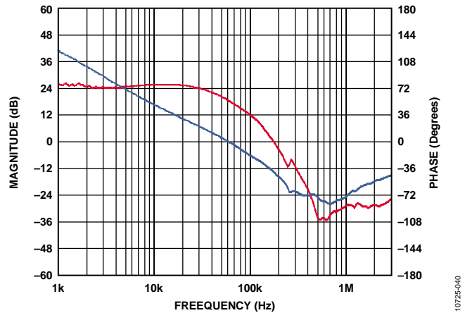
Figure 34. Bode Plot at 4 A
