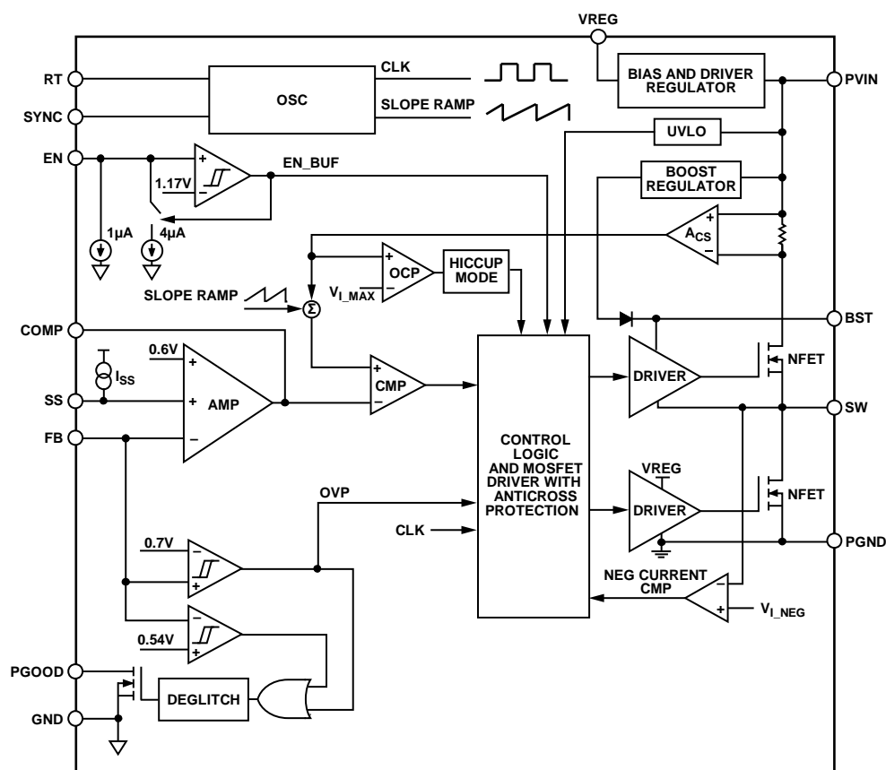
Figure 28. Functional Block Diagram
