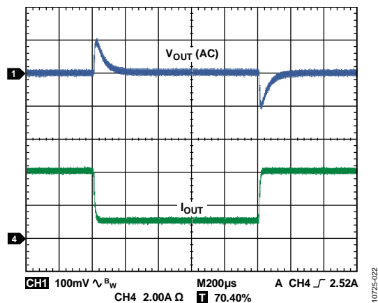
Figure 22. Load Transient Response, 1 A to 4 A
