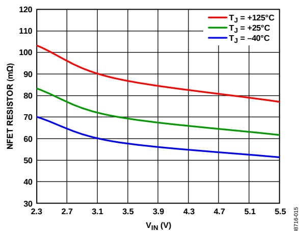
Figure 15. NFET Resistor vs. V_{IN} (Pin-to-Pin Measurements)
