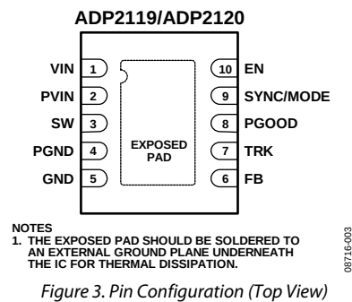
Figure 3. Pin Configuration (Top View)
