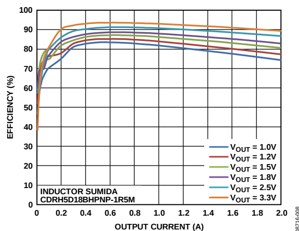
Figure 8. Efficiency (ADP2119, V_{IN} = 5\text{ V} , PFM) vs. Output Current
