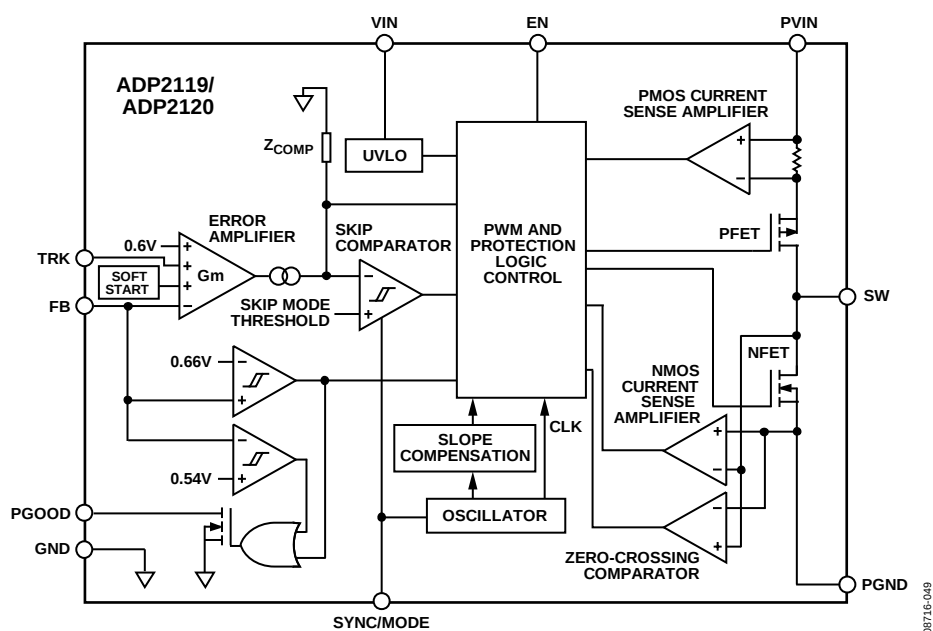
Figure 49. Functional Block Diagram
