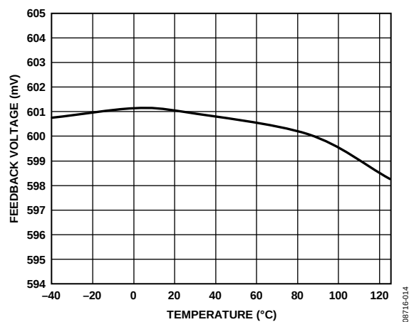
Figure 14. Feedback Voltage vs. Temperature ( V_{IN} = 3.3 V)
