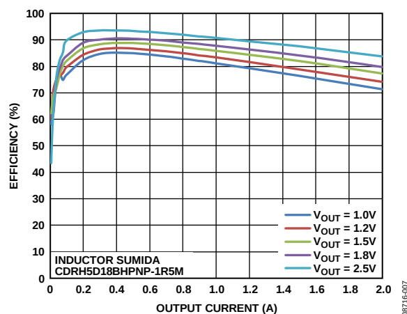
Figure 7. Efficiency (ADP2119, V_{IN} = 3.3\text{ V} , PFM) vs. Output Current
