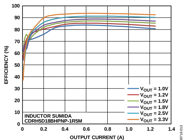
Figure 13. Efficiency (ADP2120, V_{IN} = 5 V, PFM) vs. Output Current
