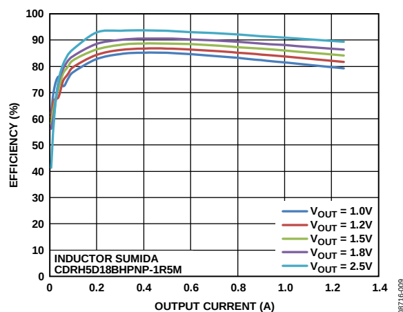
Figure 9. Efficiency (ADP2120, V_{IN} = 3.3\text{ V} , PFM) vs. Output Current
