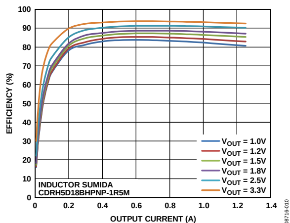
Figure 10. Efficiency (ADP2120, V_{IN} = 5 V, FPWM) vs. Output Current
