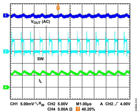
Figure 23. Steady Waveform
