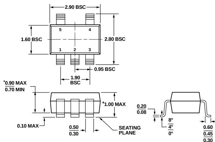
Figure 53. 5-Lead Thin Small Outline Transistor Package [TSOT] (UJ-5) Dimensions shown in millimeters
