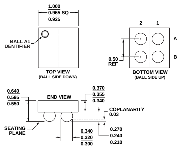
Figure 54. 4-Ball Wafer Level Chip Scale Package [WLCSP] (CB-4-1) Dimensions shown in millimeters
