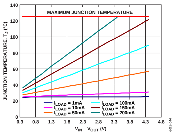
Figure 46. 100 mm² of PCB Copper, TSOT, T_A = 25^\circ\text{C}
