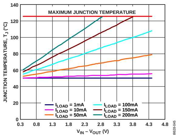
Figure 47. 500 mm² of PCB Copper, TSOT, T_A = 50^\circ\text{C}
