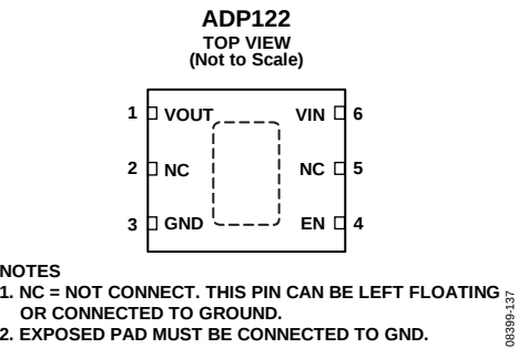
Figure 6. ADP122 LFCSP Fixed Output Pin Configuration
