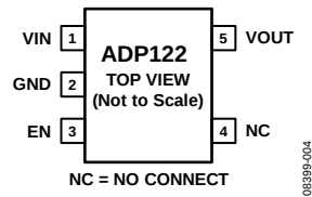
Figure 5. ADP122 TSOT Fixed Output Pin Configuration
