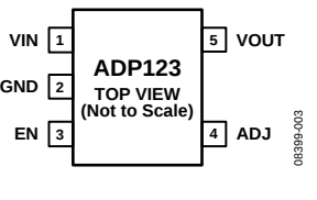
Figure 7. ADP123 TSOT Adjustable Output Pin Configuration
