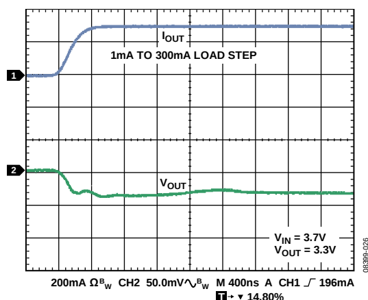
Figure 32. Output Transient Response, C_{OUT} = 1\ \mu\text{F}
