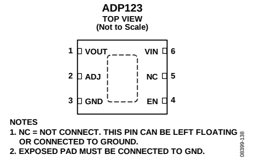
Figure 8. ADP123 LFCSP Adjustable Output Pin Configuration
