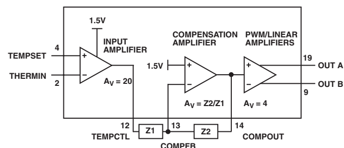
Figure 2. Signal Flow Block Diagram of the ADN8830
