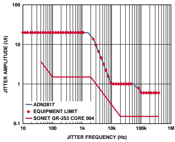
Figure 10. Jitter Tolerance, OC-1
