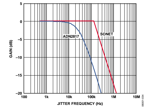
Figure 8. Jitter Transfer, OC-3
