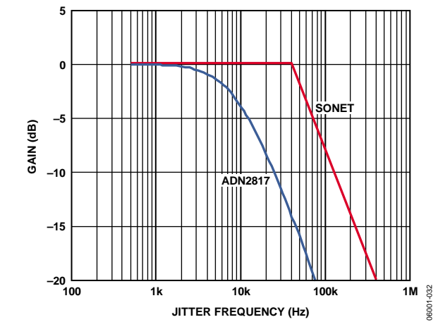
Figure 7. Jitter Transfer, OC-1
