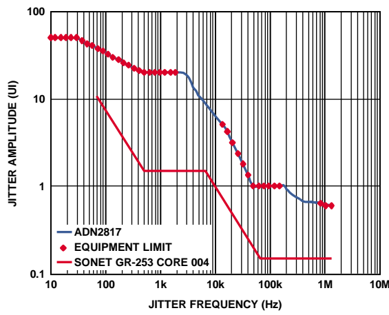
Figure 11. Jitter Tolerance, OC-3
