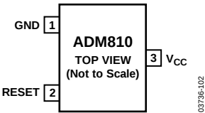
Figure 4. ADM810 Pin Configuration
