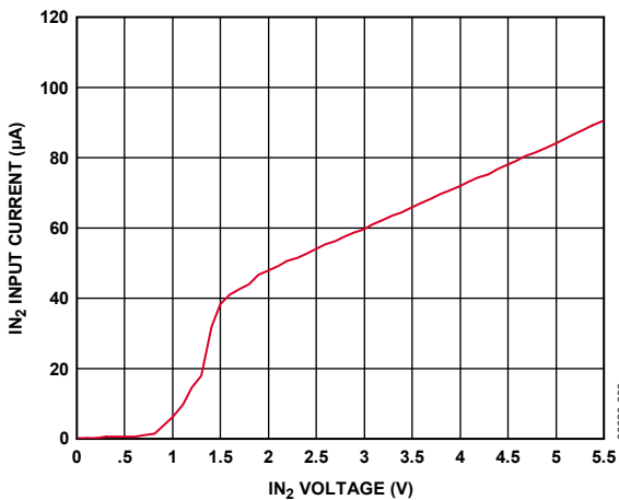
Figure 5. I_{IN2} Input Current vs. I_{IN2} Voltage
