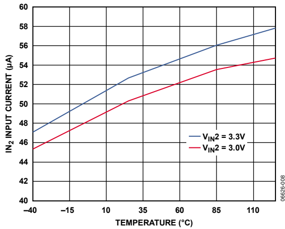
Figure 4. I_{IN2} Input Current vs. Temperature
