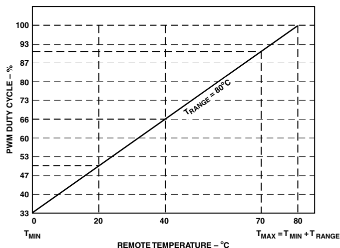
Figure 9. Max Speed Calculated by Local and Remote Temperature Control Loops Drives Fan
