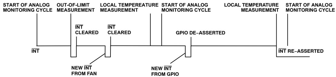
Figure 50. Other Interrupt Sources Can Reassert \overline{\text{INT}} Immediately
