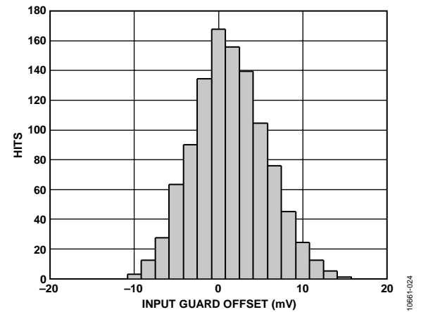
Figure 24. Distribution of Input Guard Offset Voltage V_{OLFS} ( V_{INPT} - V_{SUM} )
