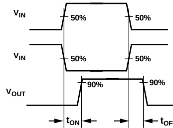
Figure 14. Switching Timing
