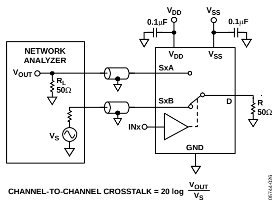
Figure 19. Channel-to-Channel Crosstalk
