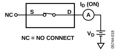
Figure 13. On Leakage
