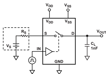
Figure 28. Charge Injection
