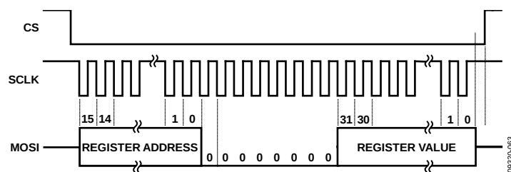
Figure 69. SPI Write
