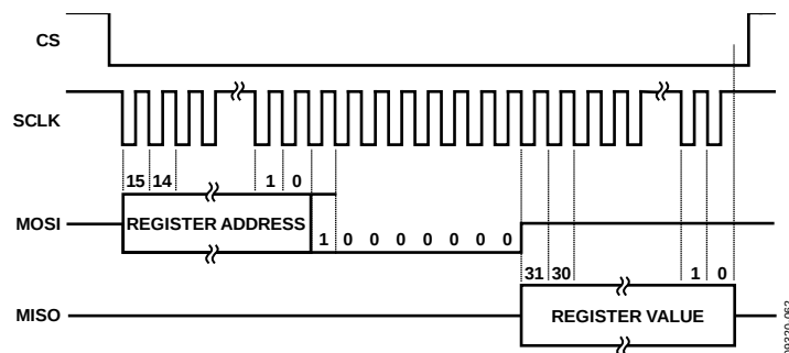
Figure 68. SPI Read
