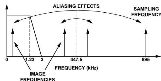
Figure 38. Aliasing Effect
