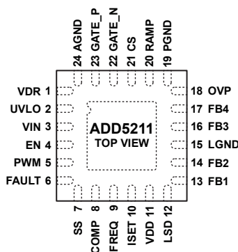
Figure 3. Pin Configuration
