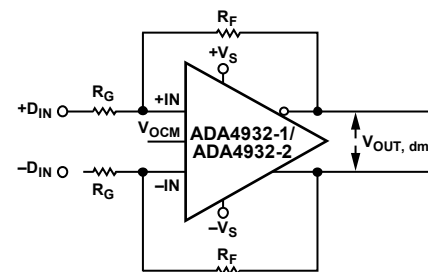
Figure 56. ADA4932-1/ADA4932-2 Configured for Balanced (Differential) Inputs
