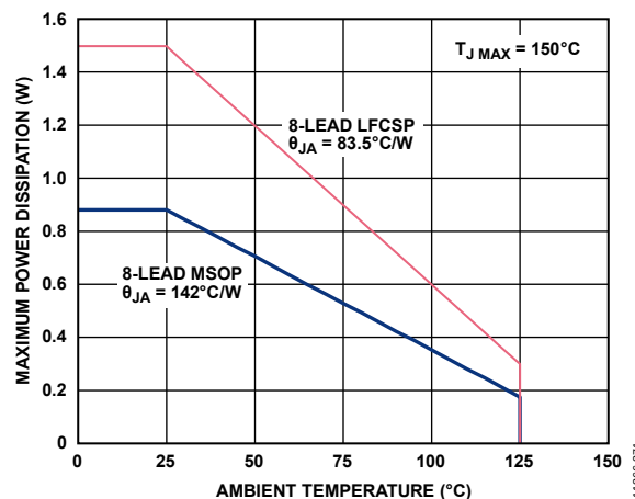
Figure 71. Maximum Power Dissipation vs. Ambient Temperature
