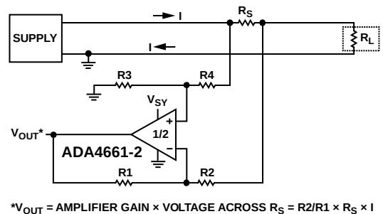
Figure 80. High-Side Current Sensing Circuit
