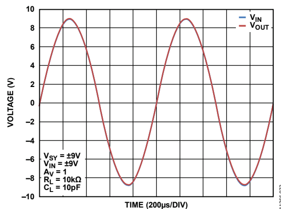
Figure 72. Rail-to-Rail Input and Output
