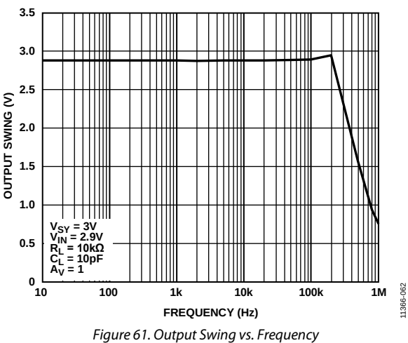
Figure 61. Output Swing vs. Frequency
