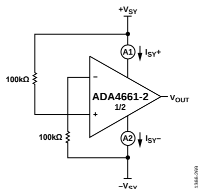
Figure 76. Comparator B
