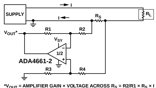
Figure 79. Low-Side Current Sensing Circuit
