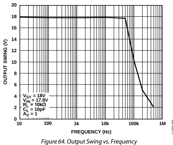
Figure 64. Output Swing vs. Frequency
