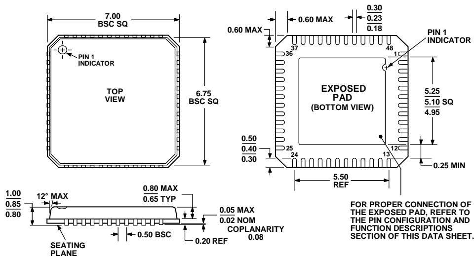
COMPLIANT TO JEDEC STANDARDS MO-220-VKGD-2 Figure 60. 48-Lead Lead Frame Chip Scale Package [LFCSP_VQ] 7 mm x 7 mm Body, Very Thin Quad (CP-48-1) Dimensions shown in millimeters
