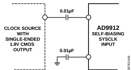
Figure 37. SYSCLK Single-Ended Input, Non-Xtal
