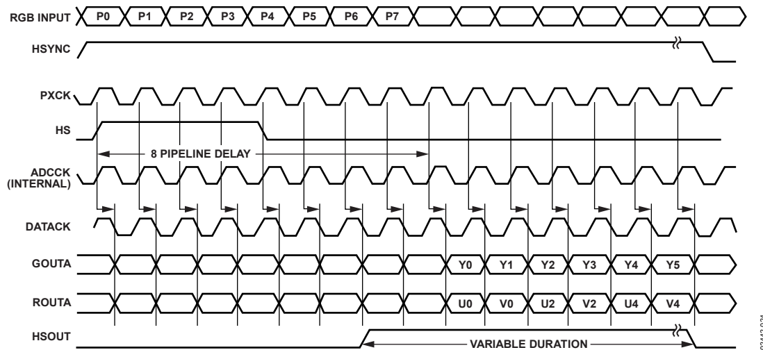
Figure 25. 4:2:2 Output Mode
