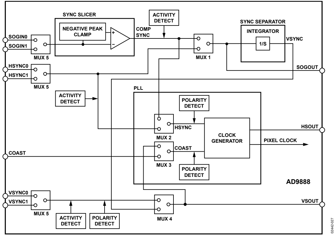
Figure 27. Sync Processing Block Diagram
