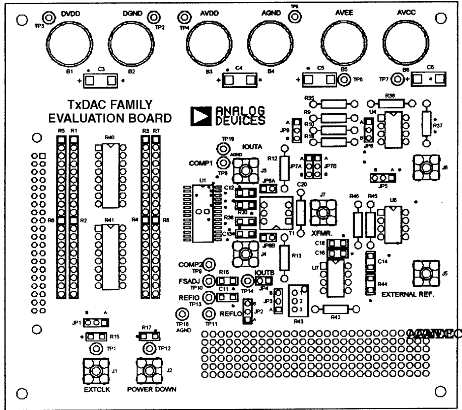
Figure 60. Silkscreen Layer—Top
